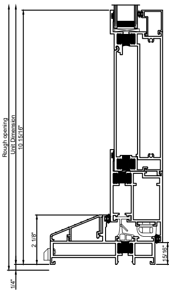
Standard Sill 10"
