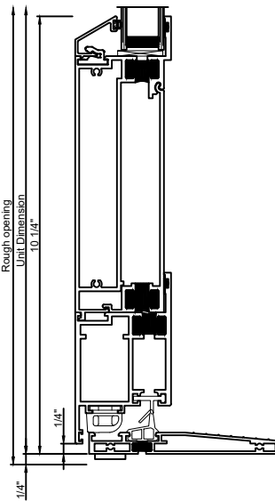
Low Profile Sill 10"
